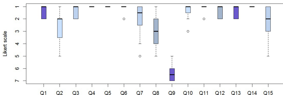
Fig.1 - Perception Results
